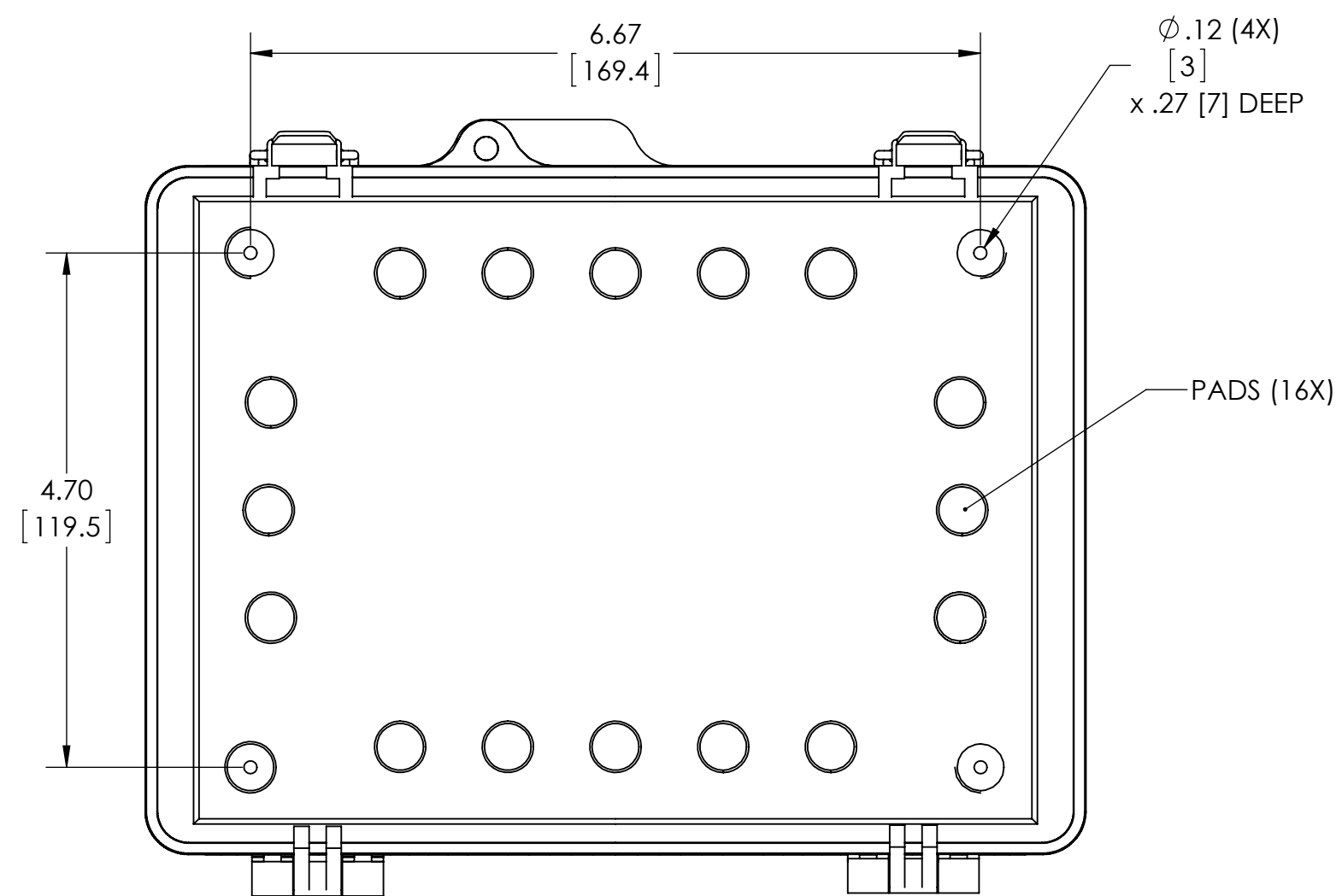
BOTTOM VIEW
