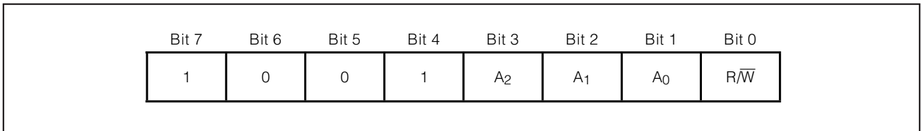
Figure 7. Address Byte
