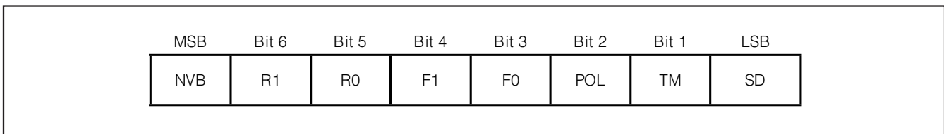
Figure 5. Configuration Register
