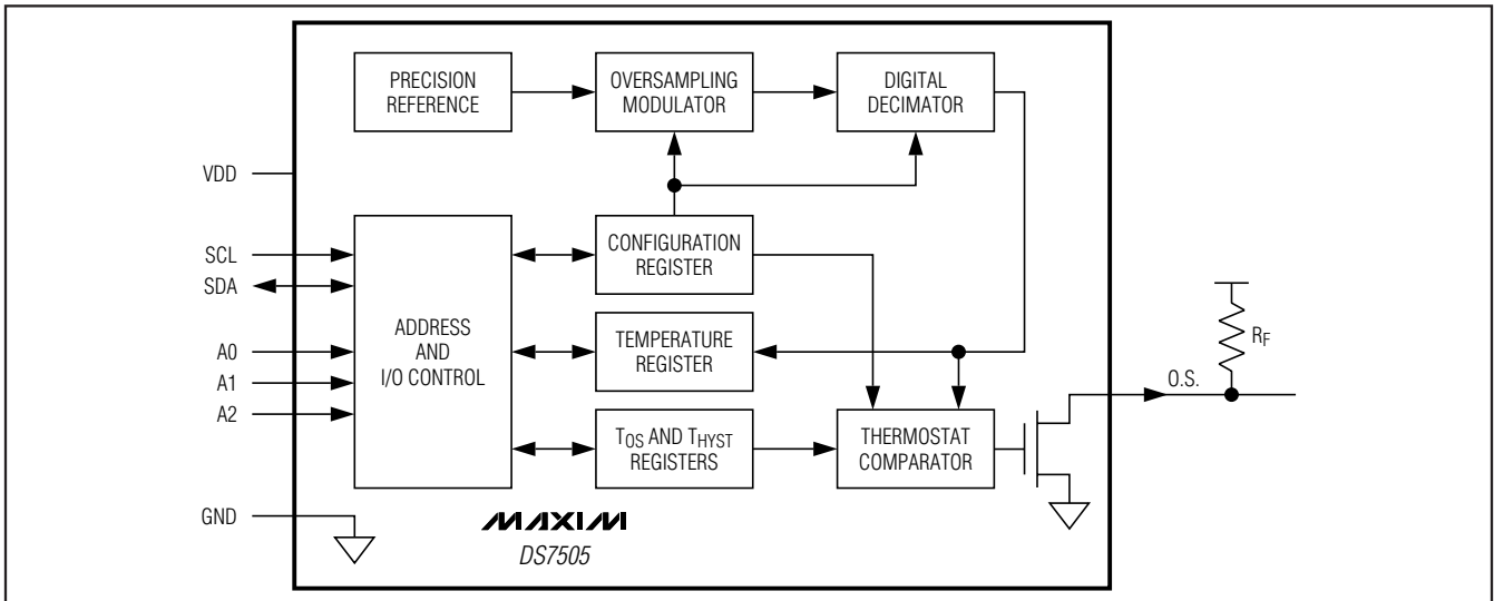
Figure 2. Block Diagram
