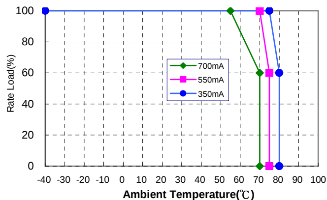
DIM01HXXW Derating Curve
