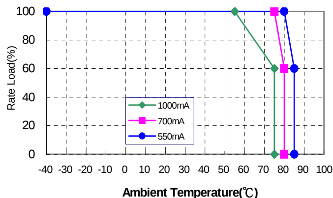
DIM01H Derating Curve
