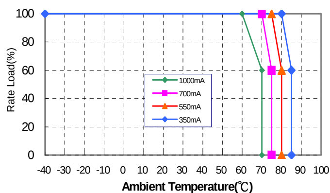
DIM01HXXW Derating Curve
