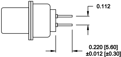
SIGNAL CONTACTS
