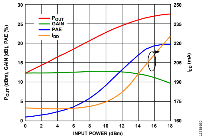
Figure 30. Power Compression at 20 GHz
