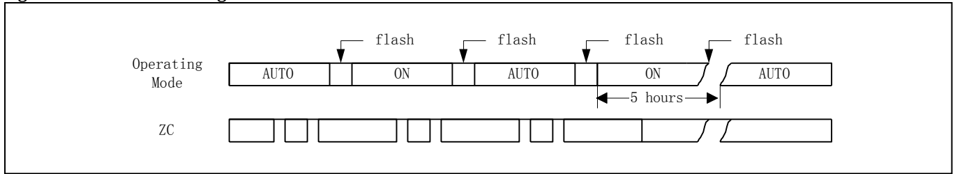
Figure 7 ZC override timing
