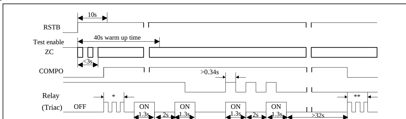
Figure 6 Test mode
