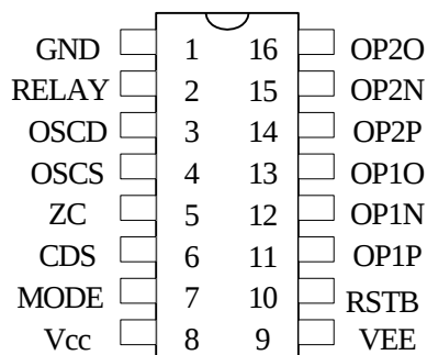
PT8A2642P/2642W
