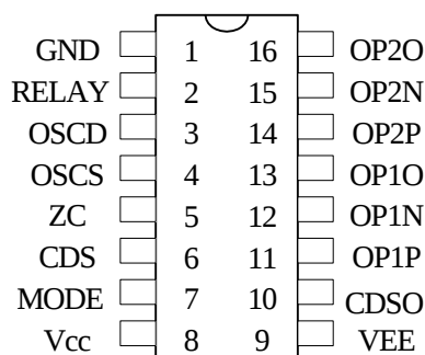
PT8A2646P/2646W
