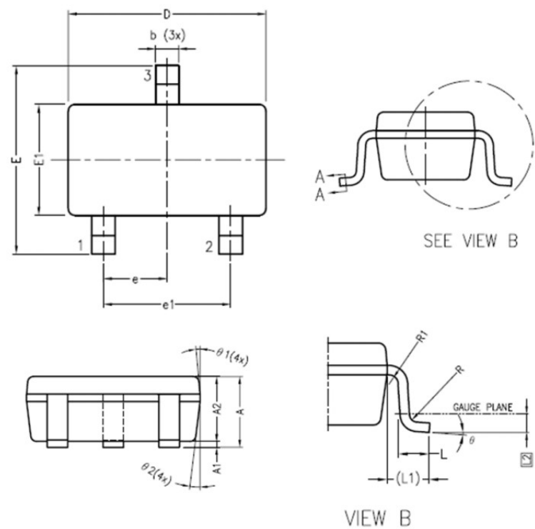
Figure 4: Package Dimensions
