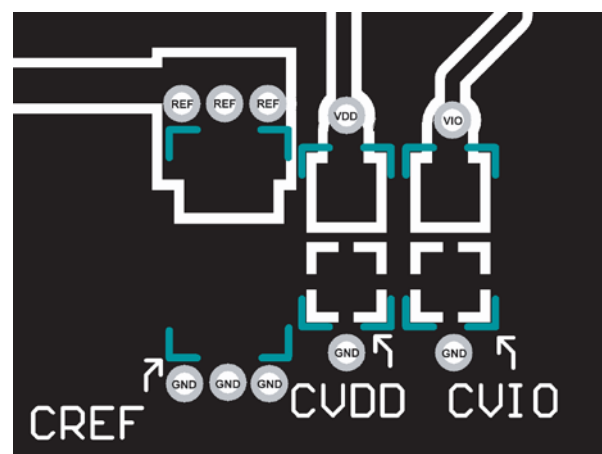
Figure 43. Example Layout of the AD7988-x (Bottom Layer)
