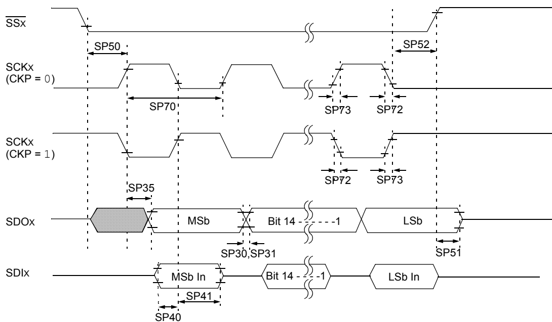
FIGURE 26-17: SPIx SLAVE MODE (FULL-DUPLEX, CKE = 0, CKP = 1, SMP = 0) TIMING CHARACTERISTICS FOR dsPIC33FJ16(GP/MC)10X
