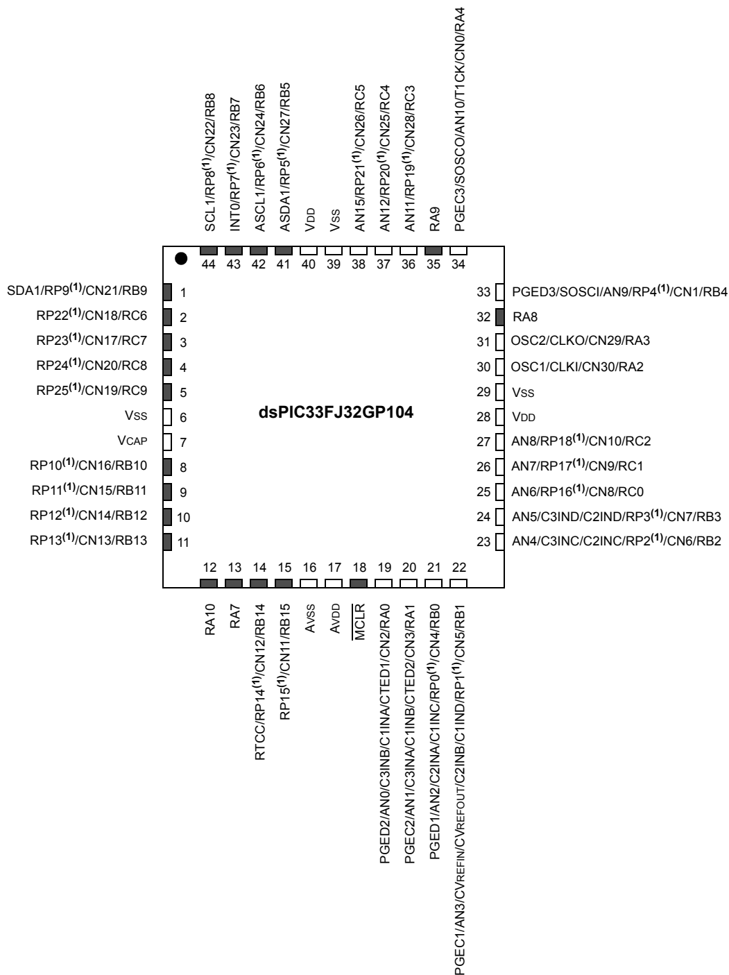
44-Pin QFN (2)
