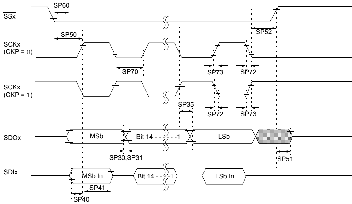
FIGURE 26-15: SPIx SLAVE MODE (FULL-DUPLEX, CKE = 1, CKP = 0, SMP = 0) TIMING CHARACTERISTICS FOR dsPIC33FJ16(GP/MC)10X
