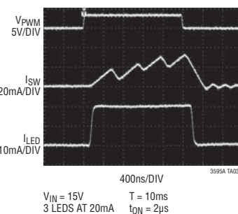
5000:1 PWM Dimming at 100Hz
