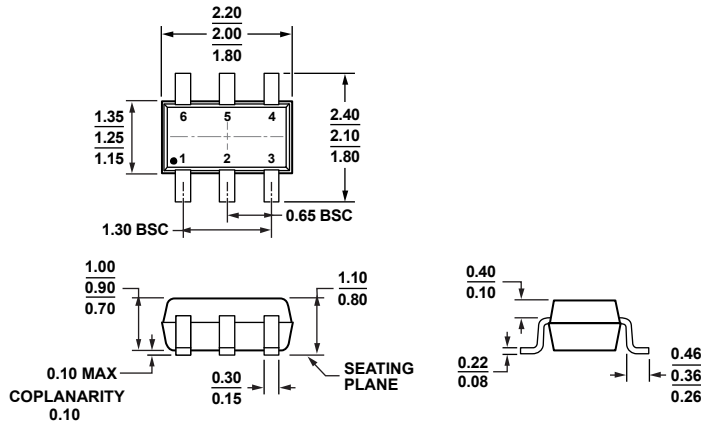
COMPLIANT TO JEDEC STANDARDS MO-203-AB Figure 32. 6-Lead Thin Shrink Small Outline Transistor Package [SC70] (KS-6) Dimensions shown in millimeters
