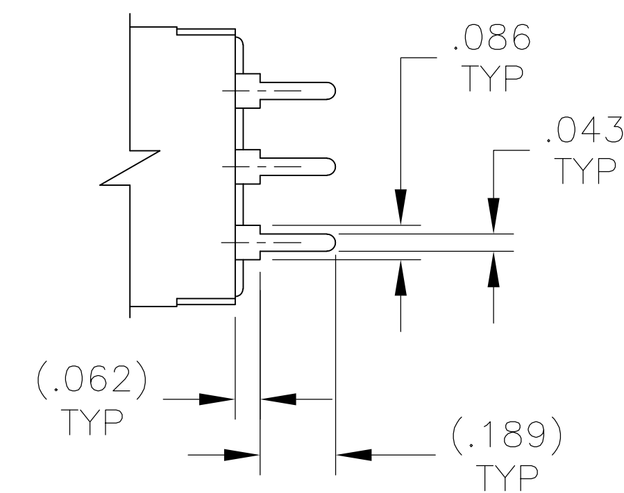
PC TERMINAL
