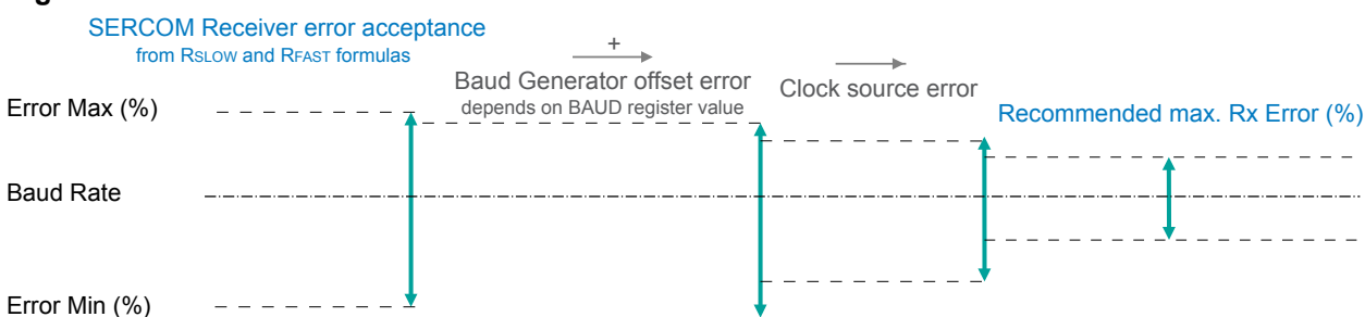
Figure 28-5. USART Rx Error Calculation
