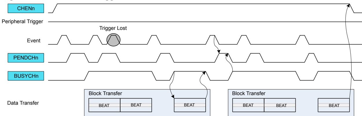
Figure 22-11. Beat Event Trigger Action
