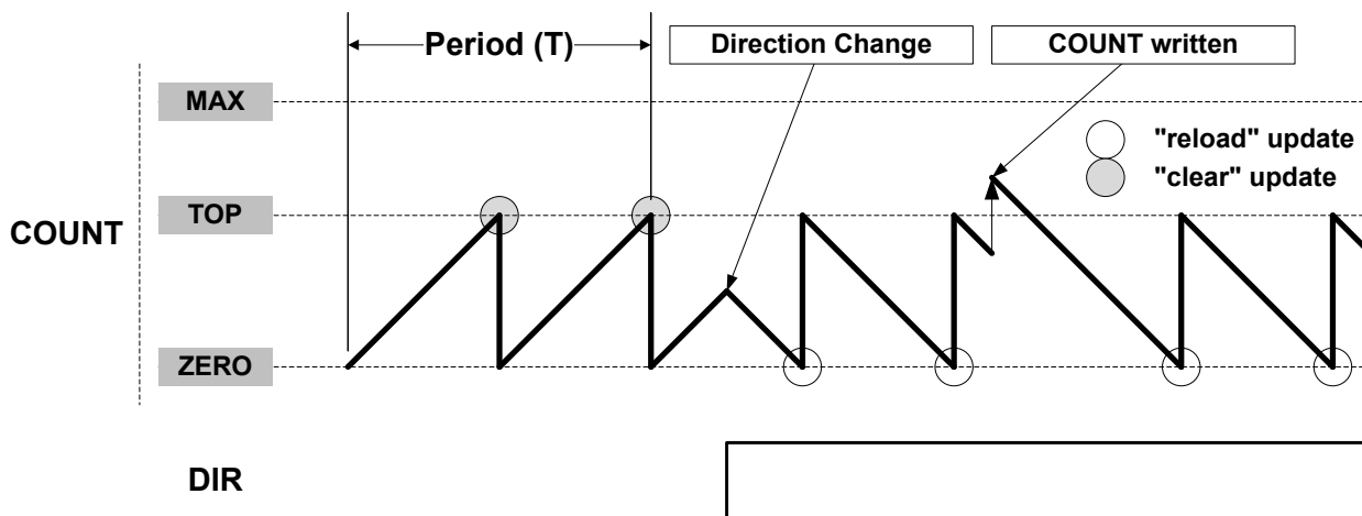
Figure 32-3. Counter Operation
