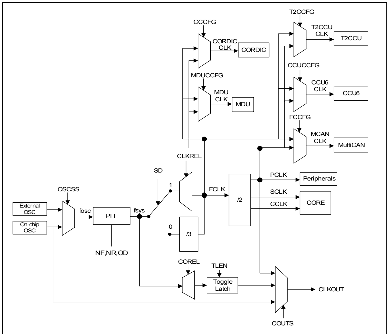
Figure 22 Clock Generation from f_{\text{sys}}
