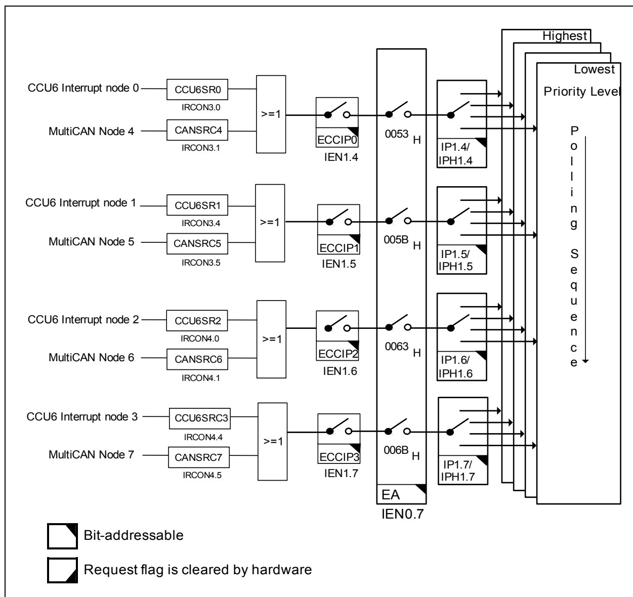
Figure 17 Interrupt Request Sources (Part 5)
