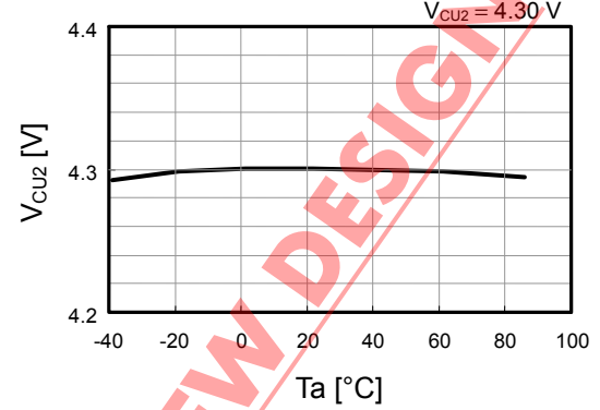
Overcharge detection voltage2 vs. temperature
