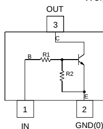
Device Schematic
