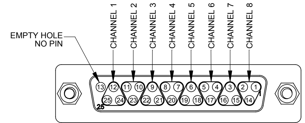
DB25F PIN-OUT VIEW
