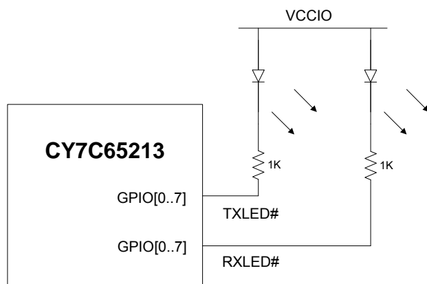
Figure 10. Double-LED Configuration
