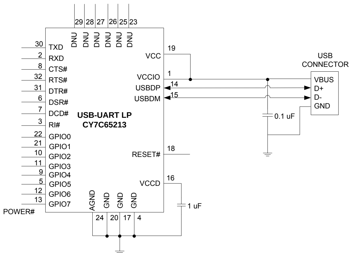
Figure 1. Bus-Powered Configuration
