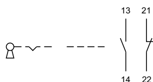
13 Keylock switch 2 positions page 9
