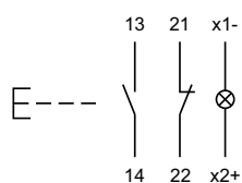
11 Illuminated pushbutton actuator page 7 | Mushroom-head pushbutton actuator page 8
