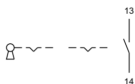
15 Keylock switch 2 positions page 9
