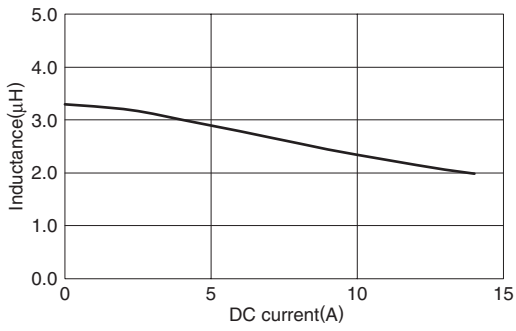
SPM6530T-3R3M
