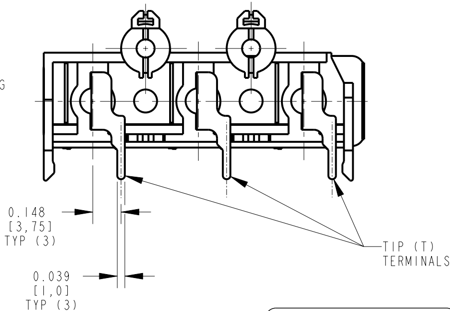
CUSTOMER DRAWING
