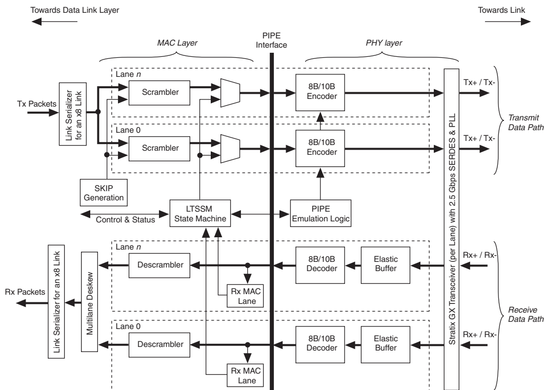
Figure 3-4. Physical Layer
