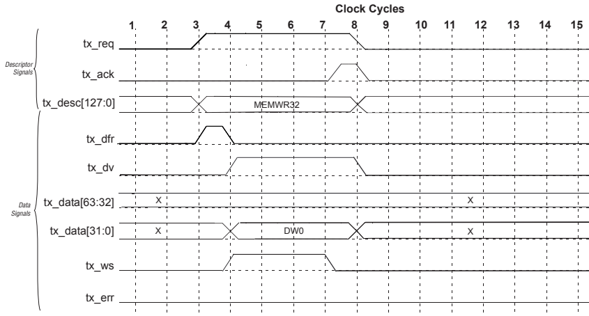
Figure 3–16. Transaction Layer Not Ready to Accept Packet
