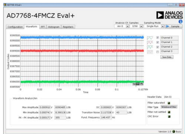
Figure 18. Waveform Tab
