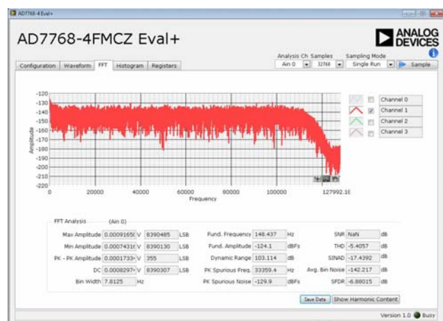
Figure 19. FFT Tab
