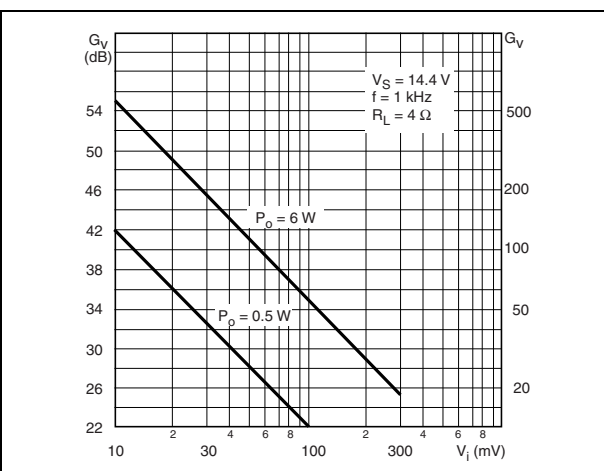
Figure 15. Gain vs. input sensitivity
