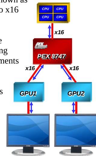
Figure 3. Dual Graphics Fan-Out
