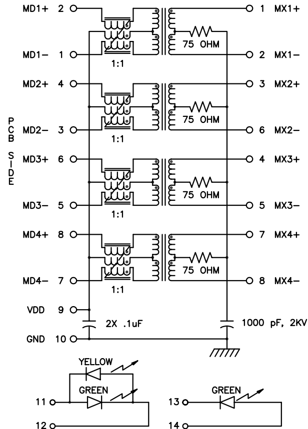
SCHEMATIC EACH PORT (2 PLACES)
