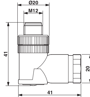
Dimensioned drawing
