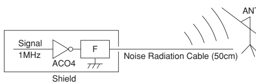
Test Circuit
