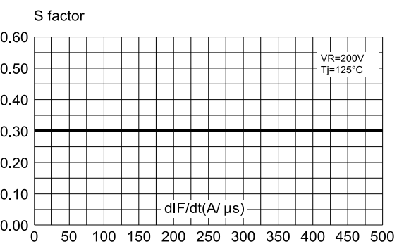
Figure 6: Softness factor versus dIF/dt (typical values)
