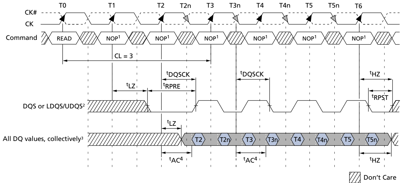
Figure 32: Data Output Timing – t_{AC} and t_{DQSCK}
