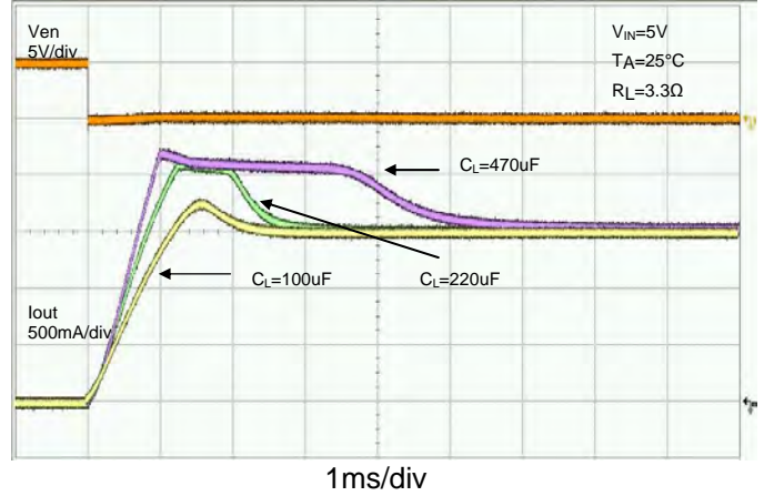
Inrush Current
