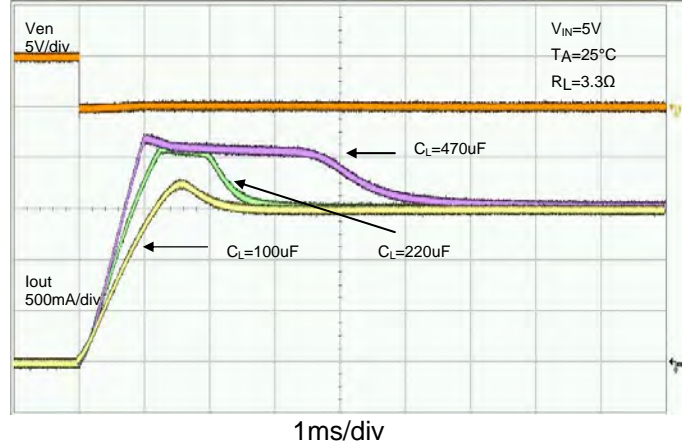
Inrush Current
