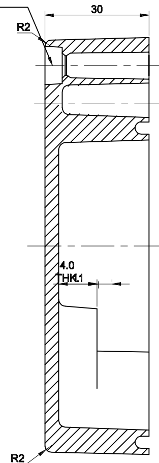
SECTION -B-B
