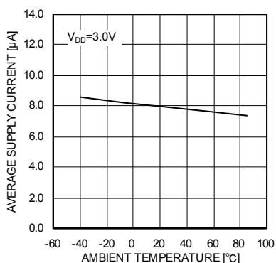
Fig.52 I_{DD} - Ambient temperature
