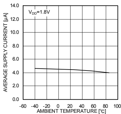
Fig.46 I_{DD} - Ambient temperature
