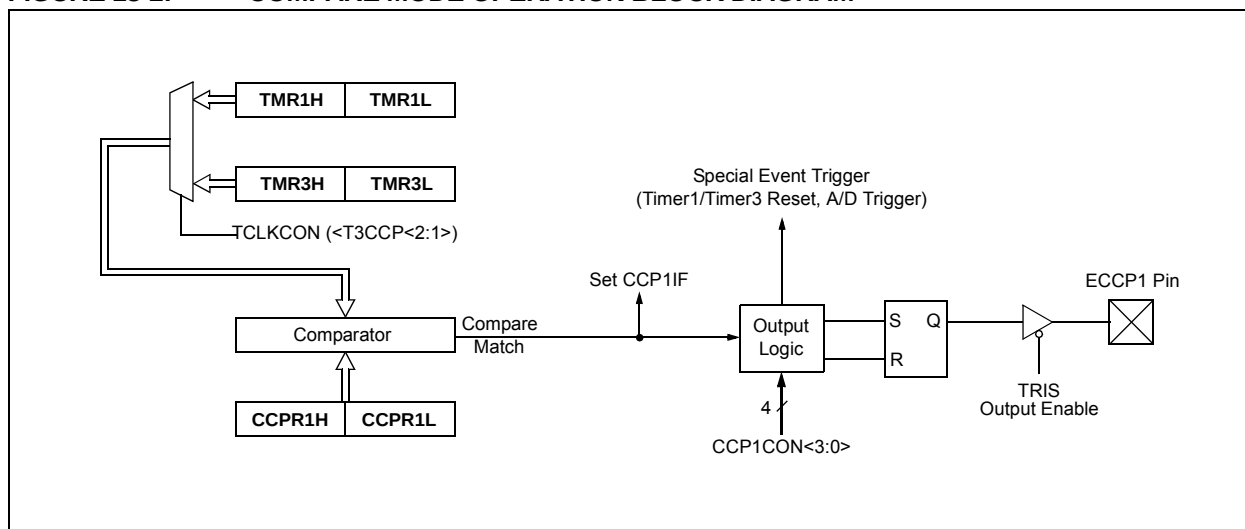
FIGURE 18-2: COMPARE MODE OPERATION BLOCK DIAGRAM
