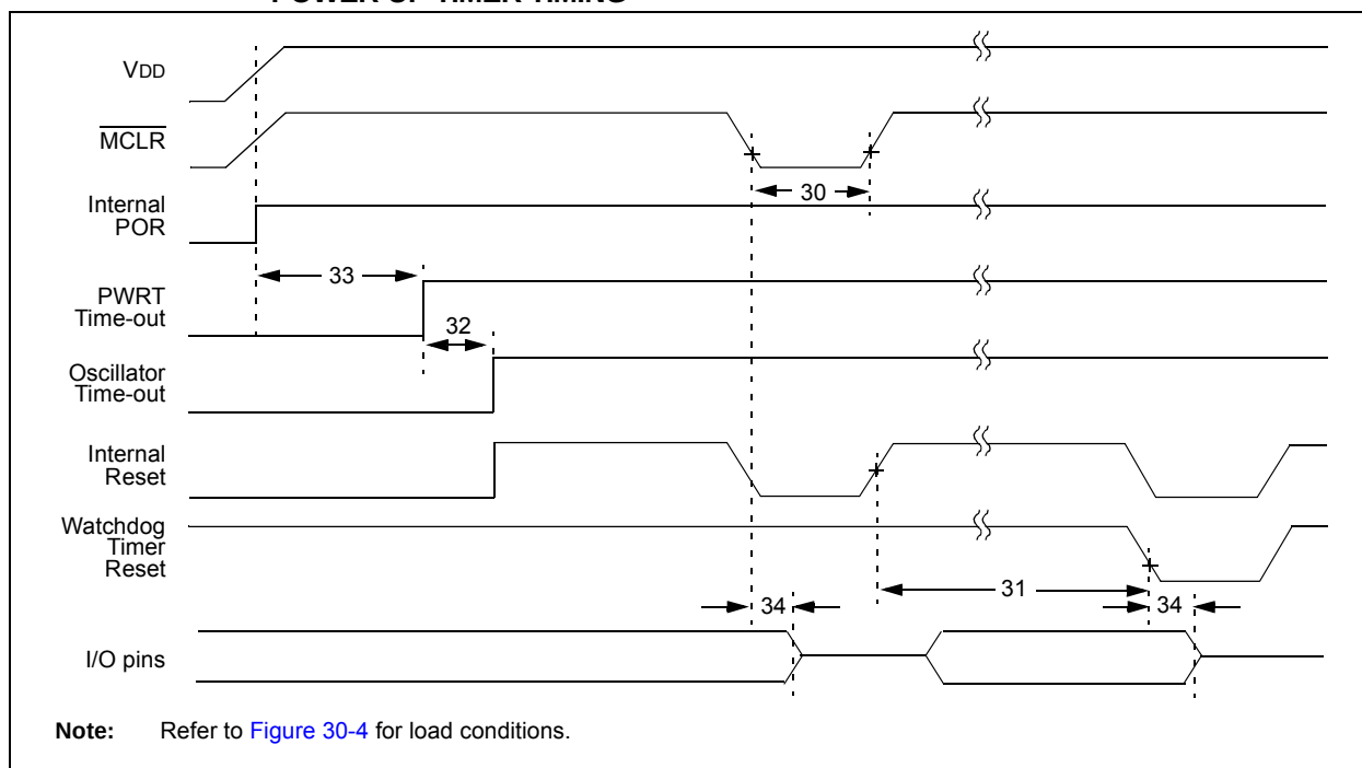
FIGURE 30-7: RESET, WATCHDOG TIMER, OSCILLATOR START-UP TIMER AND POWER-UP TIMER TIMING
