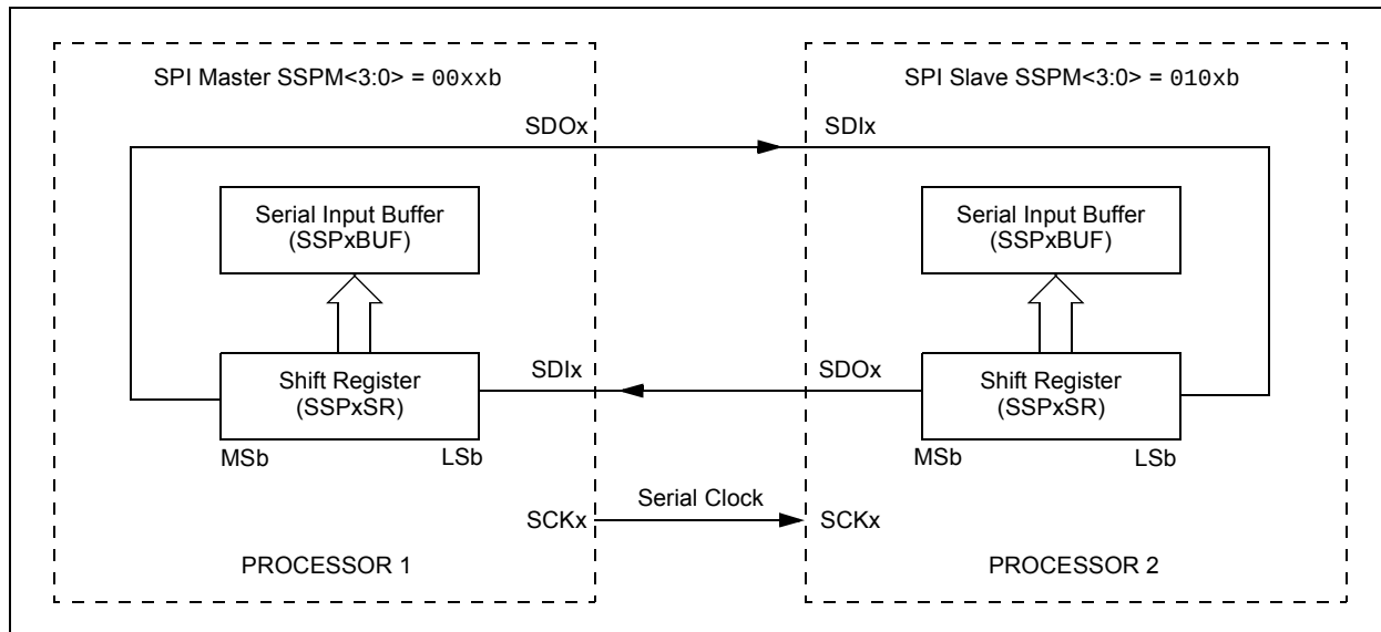
FIGURE 19-2: SPI MASTER/SLAVE CONNECTION
