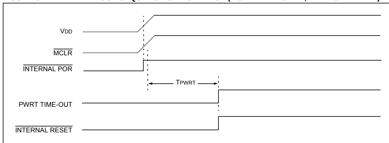
FIGURE 5-2: TIME-OUT SEQUENCE ON POWER-UP ( \overline{\text{MCLR}} TIED TO \text{V}_{\text{DD}} , \text{V}_{\text{DD}} RISE < \text{TPWRT} )
