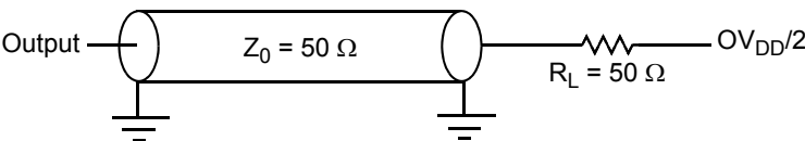
Figure 39. AC Test Load for the JTAG Interface
