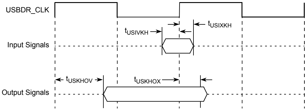
Figure 29. USB Signals
