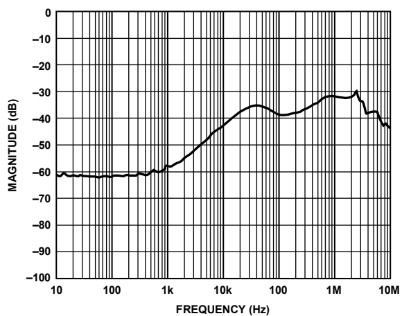
Figure 8. ADC 1.82 V Voltage Reference, AC PSRR
