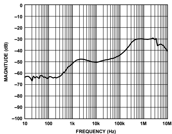
Figure 9. Low Power 2.5 V Voltage Reference, AC PSRR
