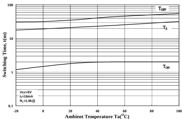
Figure 17. Switching Time vs. Ambient Temperature
