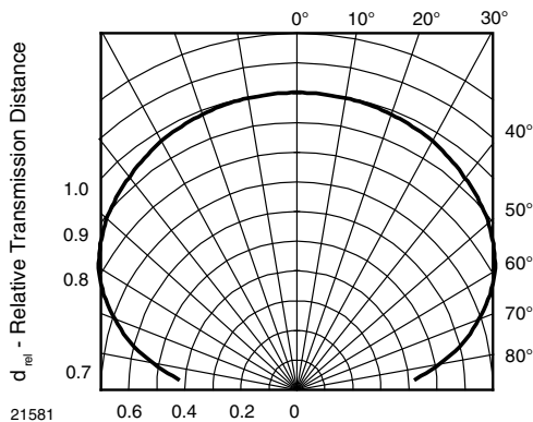
Fig. 12 - Horizontal Directivity
