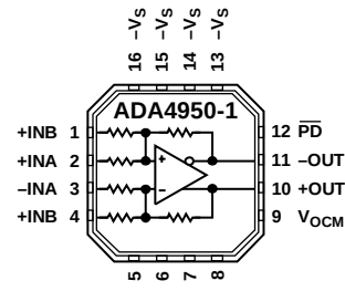
Figure 1. ADA4950-1
