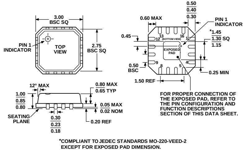
Figure 64. 16-Lead Lead Frame Chip Scale Package [LFCSP_VQ] 3 mm × 3 mm Body, Very Thin Quad (CP-16-2) Dimensions shown in millimeters
