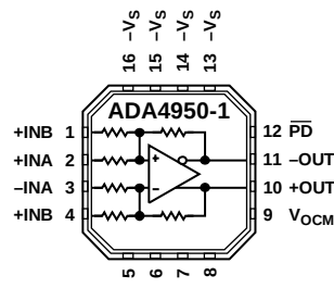
Figure 1. ADA4950-1
