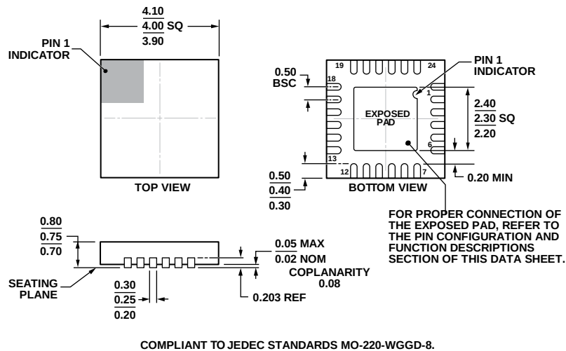
Figure 65. 24-Lead Lead Frame Chip Scale Package [LFCSP_WQ] 4 mm × 4 mm Body, Very Very Thin Quad (CP-24-14) Dimensions shown in millimeters
