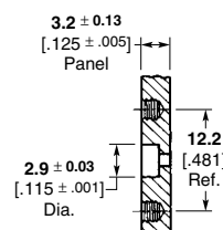
Detail D*
