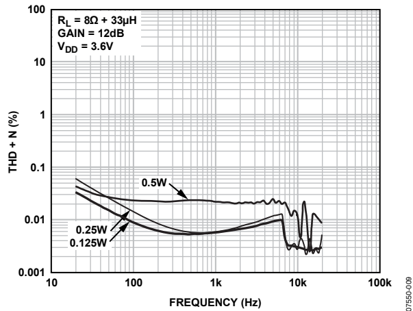
Figure 9. THD + N vs. Frequency, R_L = 8\Omega + 33\mu H , Gain = 12 dB, V_{DD} = 3.6\text{ V}
