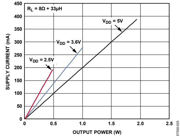
Figure 25. Supply Current vs. Output Power into R_L = 8\ \Omega + 33\ \mu\text{H}
