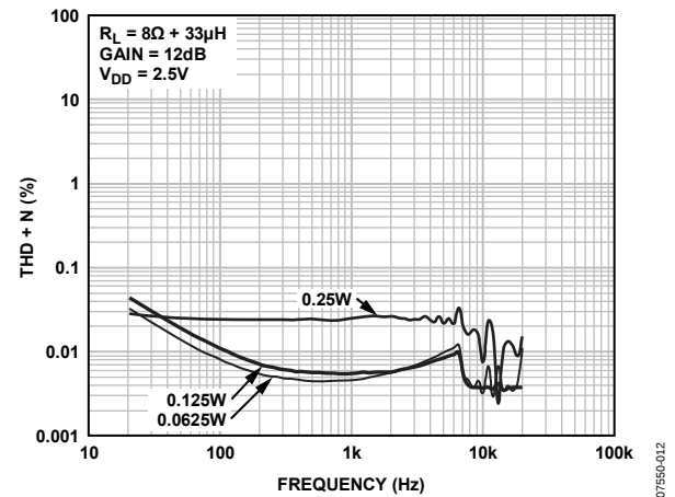
Figure 12. THD + N vs. Frequency, R_L = 8\Omega + 33\mu H , Gain = 12 dB, V_{DD} = 2.5\text{ V}
