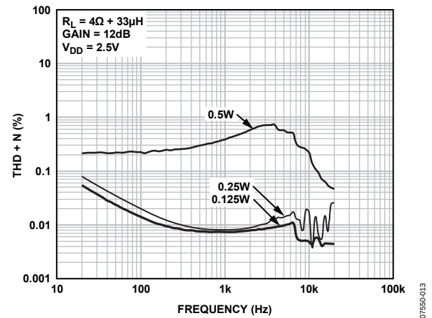
Figure 13. THD + N vs. Frequency, R_L = 4\Omega + 33\mu H , Gain = 12 dB, V_{DD} = 2.5\text{ V}
