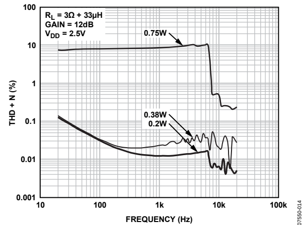
Figure 14. THD + N vs. Frequency, R_L = 3\Omega + 33\mu H , Gain = 12 dB, V_{DD} = 2.5\text{ V}
