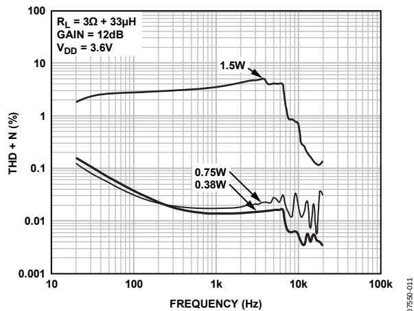
Figure 11. THD + N vs. Frequency, R_L = 3\Omega + 33\mu H , Gain = 12 dB, V_{DD} = 3.6\text{ V}
