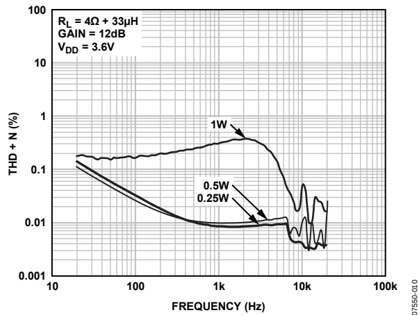
Figure 10. THD + N vs. Frequency, R_L = 4\Omega + 33\mu H , Gain = 12 dB, V_{DD} = 3.6\text{ V}
