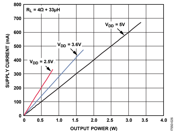
Figure 26. Supply Current vs. Output Power into R_L = 4\ \Omega + 33\ \mu\text{H}
